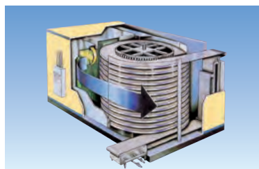
Freezer
