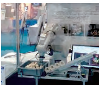
Workpieces are handled precisely
