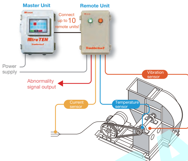
② Blower/Rotating Machine Monitoring System (Showa Denki)
